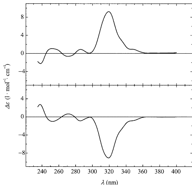
Figure 1. CD spectra of the two enantiomers [( R,R ) and ( S,S )] of 1 . For the assignment of the absolute configuration see text.
