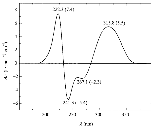
Figure 2. CD spectrum of ( R,R )- 1 calculated at the B3LYP/TZVP level of time-dependent density functional theory (TDDFT).
