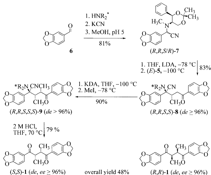
Scheme 2. First asymmetric synthesis of the Virola sebifera lignan ( S,S )- 1 .
