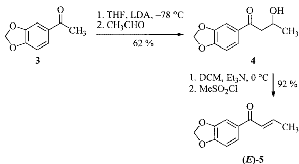
Scheme 1. Synthesis of the enone Michael acceptor ( E )- 5 .
